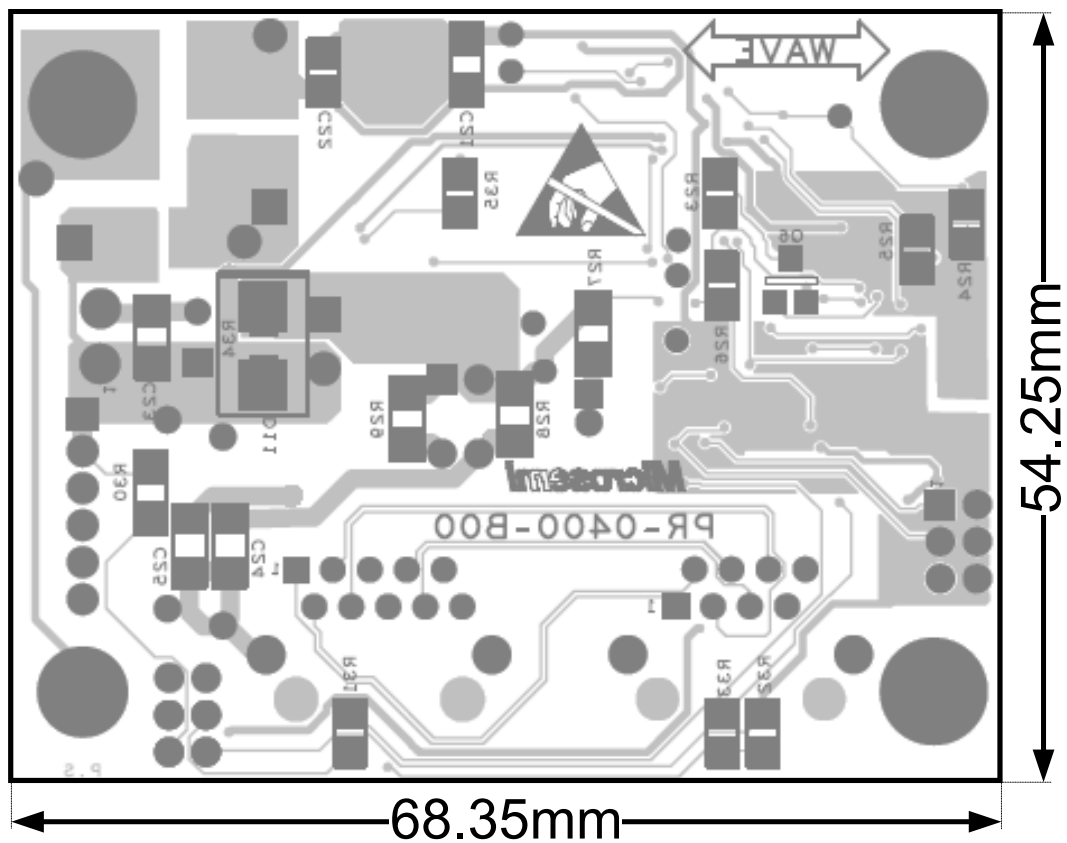
Figure 3: Layout Example of Component and Print Side
